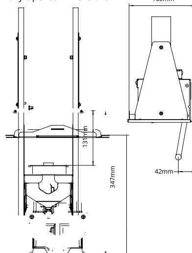
Fully Opened Dimensions
