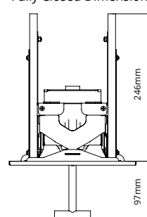
Fully Closed Dimensions
