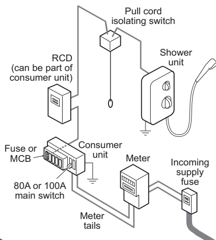
Fig.4 Schematic of installation circuit
